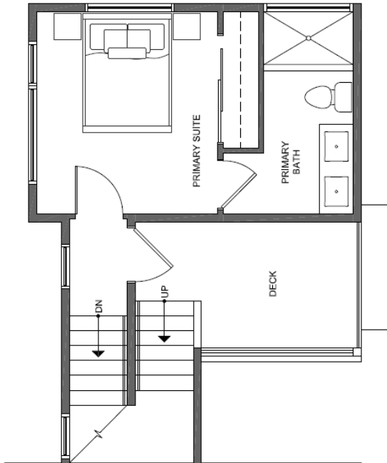
FLOOR 3 (SFR & ADU)
