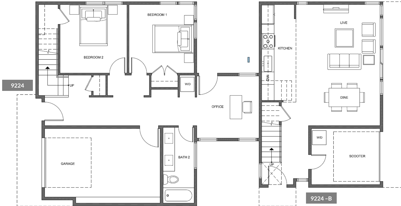
FLOOR 1 (SFR & ADU)
