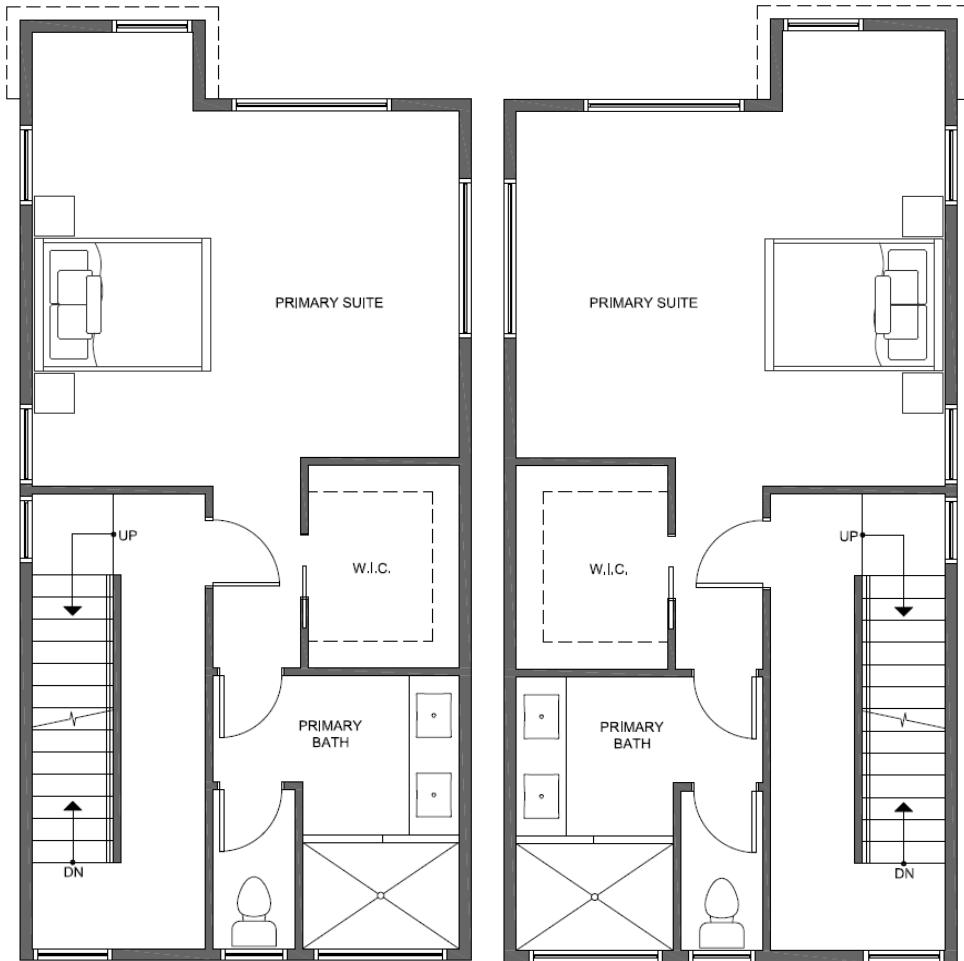
FLOOR 3
